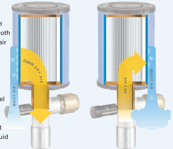
Figure 1: Inhale and exhale cycles of a Donaldson breather, moisture and contaminant is prevented from entering the tank.
